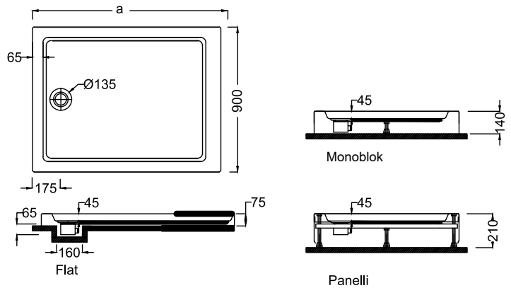
Panelli h: 21 cm
