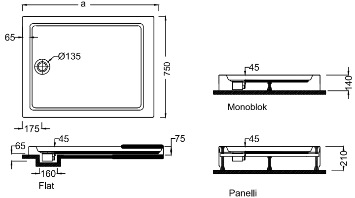
Panelli h: 21 cm
